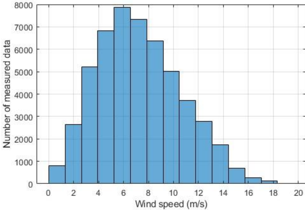
Figure 10. E01: horizontal wind speed frequency distribution at 12 m.
